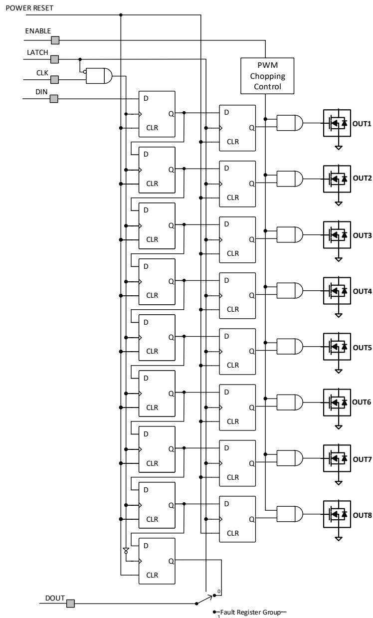
Figure 4. 8bit Shift Register
