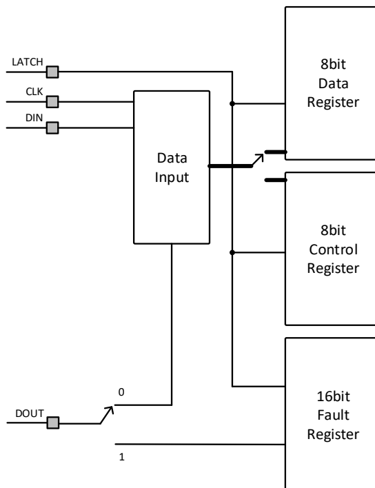
Figure 3. Register Overview
