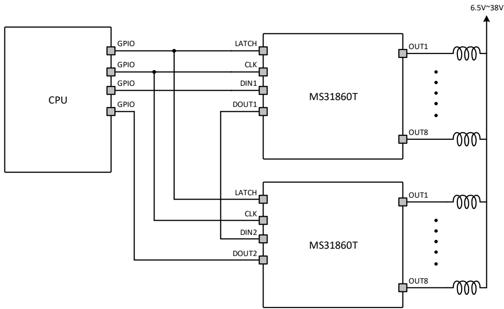
Figure 2. Multiple MS31860Ts Daisy Chain
