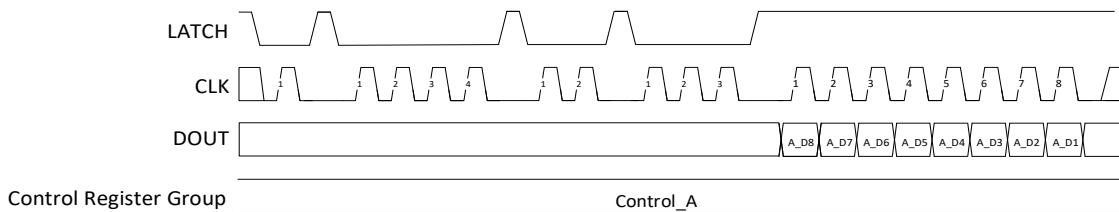
Figure 17. Read Control Register Group-Single MS31860T
