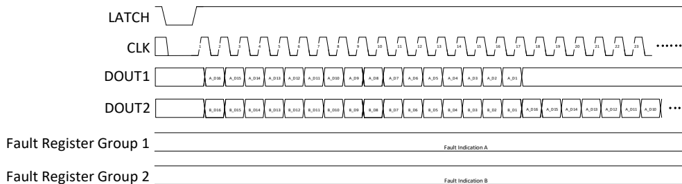
Figure 21. Read Fault Register Group-Dual MS31860Ts Daisy Chain
