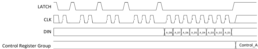
Figure 15. Write Control Register Group-Single MS31860T
